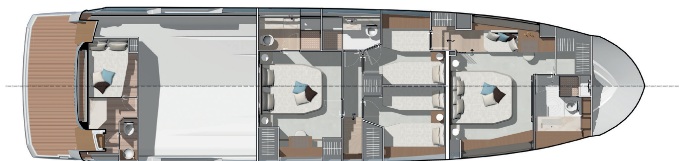
Lower deck - 4 Stateroom version
