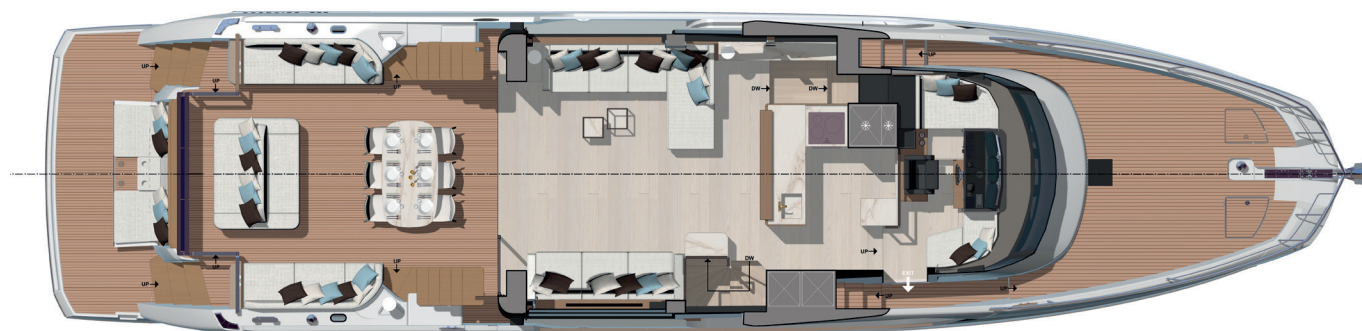
Main deck - Exterior dining version
